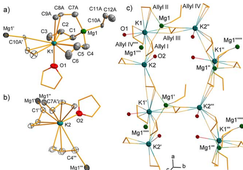
Figure 4. Cutouts of solid-state structure of [K_2Mg(C_3H_5)_4(THF)_2] \cdot ([8 \cdot (THF)_2]) . Displacement ellipsoids are shown at the 50% probability level. Hydrogen atoms are omitted for clarity, disordered carbon atoms are shown with one split position. Coordination geometries around Mg1 and K1 (a) and K2 (b). Atoms that exceed one formula unit of [8 \cdot (THF)_2] are drawn as empty ellipsoids. (c) Arrangement of ([8 \cdot (THF)_2]) as a three-dimensional coordination polymer with carbon atoms shown as wire frame ( C^{allyl} ) or omitted for clarity ( C^{THF} ). Allyl I–IV refers to C1–3, C4–6, C7–10, and C10–12, respectively. Selected bond lengths [Å] and angles [°]: Mg1–C1, 2.253(6); Mg1–C4, 2.254(6); Mg1–C7A, 2.29(2); Mg1–C7B, 2.26(3); Mg1–C10A, 2.175(18); Mg1–C10B, 2.41(4); K1–C1, 3.301(6); K1–C2, 3.144(6); K1–C3, 3.082(6); K1–C4, 3.481(7); K1–C5, 3.135(7); K1–C6, 3.044(7); K1–C7A, 3.87(3); K1–C8A, 3.155(8); K1–C9A, 3.22(7); K1–C10A, 3.242(18); K1–C11A, 3.056(9); K1–C12A, 3.18(2); K1–O1, 2.671(4); K2–C1, 3.165(6); K2–C2, 3.039(6); K2–C3, 3.243(6); K2–C4, 3.334(6); K2–C5, 3.049(8); K2–C6, 3.082(7); K2–C7A, 3.06(2); K2–C8A, 2.991(8); K2–C9A, 3.14(7); K2–O2, 2.709(4); C1–C2, 1.447(8); C2–C3, 1.311(9); C4–C5, 1.454(10); C5–C6, 1.306(11); C7A–C8A, 1.52(3); C8A–C9A, 1.37(6); C10A–C11A, 1.441(19); C11A–C12A, 1.37(2).
