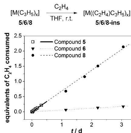
Figure 6. Course of reaction of compounds 5 , 6 , and 8 with ethylene. 5
