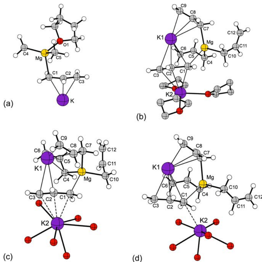
Figure 5. Calculated structures of Mg/K allyl complexes: (a) 10a [(\text{CH}_3)_2\text{Mg}(\text{THF})(\text{C}_3\text{H}_5)\text{K}] ; (b) 10b [(\text{C}_3\text{H}_5)\text{Mg}(\text{C}_3\text{H}_5)_2\text{K}(\text{C}_3\text{H}_5)\text{K}(\text{THF})_3] (hydrogen atoms have been omitted from the THF ligands for clarity); and (c) 10c and (d) 10d [(\text{C}_3\text{H}_5)\text{Mg}(\text{C}_3\text{H}_5)_2\text{K}(\text{C}_3\text{H}_5)][\text{K}(\text{THF})_6] (only the oxygen atoms of the THF ligands are shown; dotted lines represent closest approaches of the potassium to the allyl ligands).
