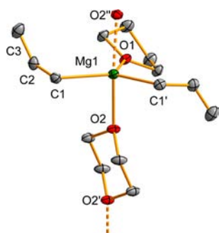
Figure 1. Molecular structure of [\text{Mg}(\eta^1\text{-C}_3\text{H}_5)_2(\text{THF})(\mu_2\text{-1,4-dioxane})] ( 2 ) in the solid state. Displacement ellipsoids are shown at the 50% probability level. Hydrogen atoms are omitted for clarity. Selected bond lengths [Å] and angles [°]: Mg1–C1, 2.2021(15); Mg1–O1, 2.0656(17); Mg1–O2, 2.2411(15); C1–C2, 1.4554(15); C2–C3, 1.3429(17); C1–Mg1–C1', 126.66(7); C1–Mg1–O1, 116.67(4); C1–Mg1–O2, 92.33(4); O2–Mg1–O2'', 163.59(5).
